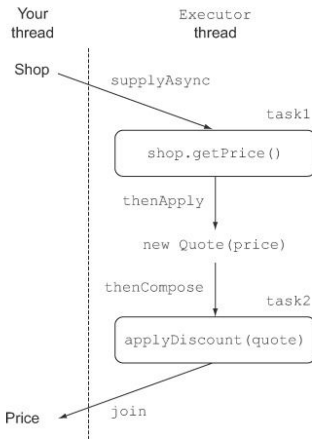
Figure 11.5. Composing synchronous operations and asynchronous tasks
