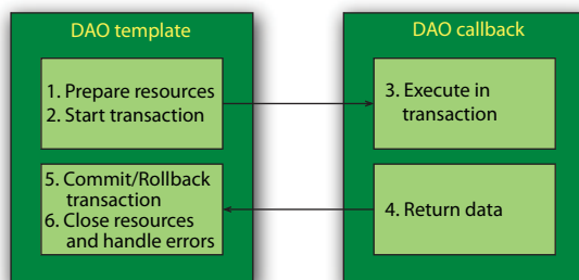
Figure 5.2 Spring's DAO template classes take responsibility for the common data access duties. For the application-specific tasks, it calls back into a custom DAO callback object.
