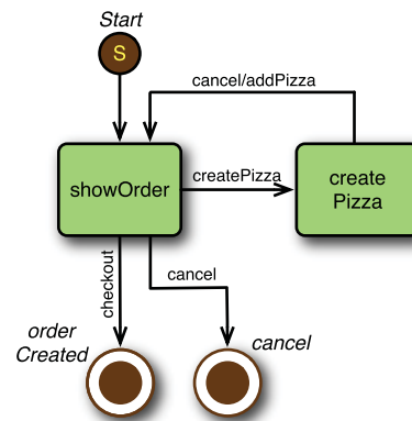
Figure 8.4 Pizzas are added via the order subflow.
