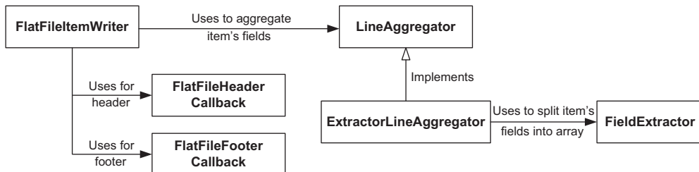
Figure 6.4 The interfaces and classes involved in writing items to a flat file with the FlatFileItemWriter . The FlatFileItemWriter also provides optional callbacks for the header and the footer of a flat file. The LineAggregator transforms an item into a string. The ExtractorLineAggregator implementation uses a FieldExtractor to “split” an item into an array of objects and calls business logic to render the array as a string.
