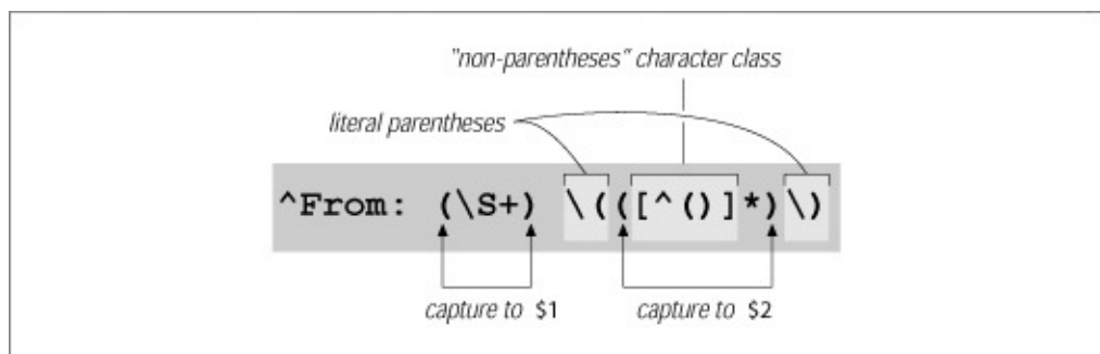
Figure 4. Nested parentheses; $1 and $2
