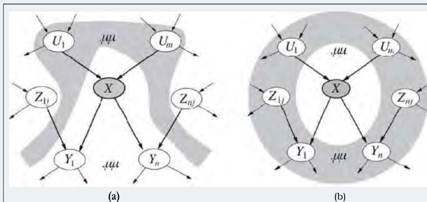
Figure 14.4 (a) A node X is conditionally independent of its non-descendants (e.g., the Z_{ij} 's) given its parents (the U_i 's shown in the gray area). (b) A node X is conditionally independent of all other nodes in the network given its Markov blanket (the gray area).
