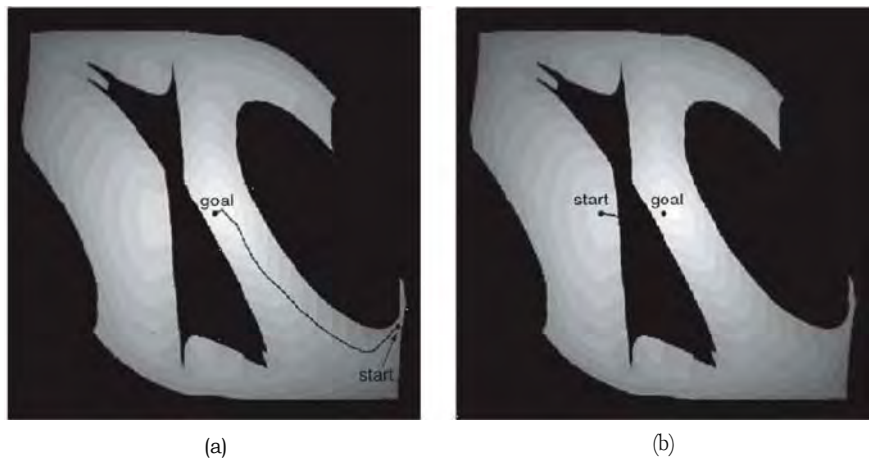
Figure 25.23 Potential field control. The robot ascends a potential field composed of repelling forces asserted from the obstacles and an attracting force that corresponds to the goal configuration. (a) Successful path. (b) Local optimum.
