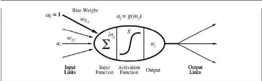
Figure 18.19 A simple mathematical model for a neuron. The unit's output activation is a_j = g(\sum_{i=0}^n w_{ij} a_i) where a_i is the output activation of unit i and w_{ij} is the weight on the link from unit i to this unit.
