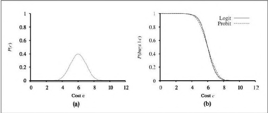
Figure 14.7 (a) A normal (Gaussian) distribution for the cost threshold, centered on \mu = 6.0 with standard deviation \sigma = 1.0 . (b) Logit and probit distributions for the probability of buys given cost, for the parameters \mu = 6.0 and \sigma = 1.0 .
