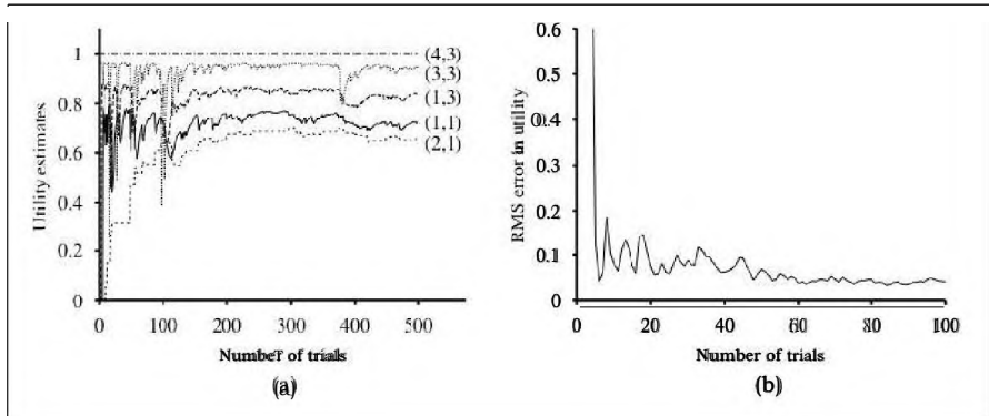
Figure 21.5 The TD learning curves for the 4 \times 3 world. (a) The utility estimates for a selected subset of states, as a function of the number of trials. (b) The run time-mean-square error in the estimate for U(1, 1) , averaged over 20 runs of 500 trials each. Only the first 100 trials are shown to enable comparison with Figure 21.3.
