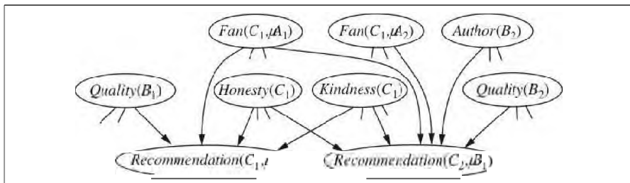
Figure 14.19 Fragment of the equivalent Bayes net when Author(B_2) is unknown.
