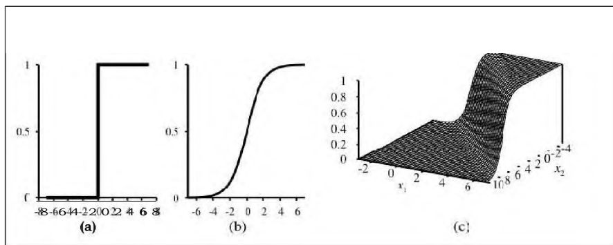
Figure 18.17 (a) The hard threshold function \text{Threshold}(z) with 0/1 output. Note that the function is nondifferentiable at z = 0 . (b) The logistic function, \text{Logistic}(z) = \frac{1}{1+e^{-z}} , also known as the sigmoid function. (c) Plot of a logistic regression hypothesis h_{\mathbf{w}}(\mathbf{x}) = \text{Logistic}(\mathbf{w} \cdot \mathbf{x}) for the data shown in Figure 18.15(b).
